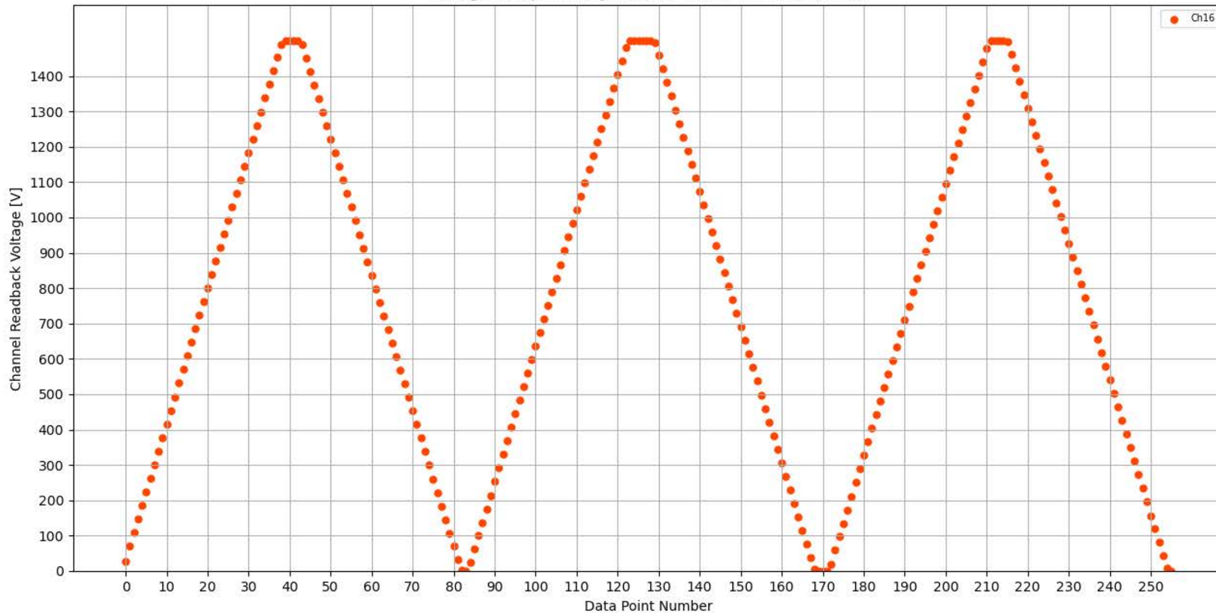
Voltage Ramp Test (Python) Bd #338, Slot #5, Ch #16
