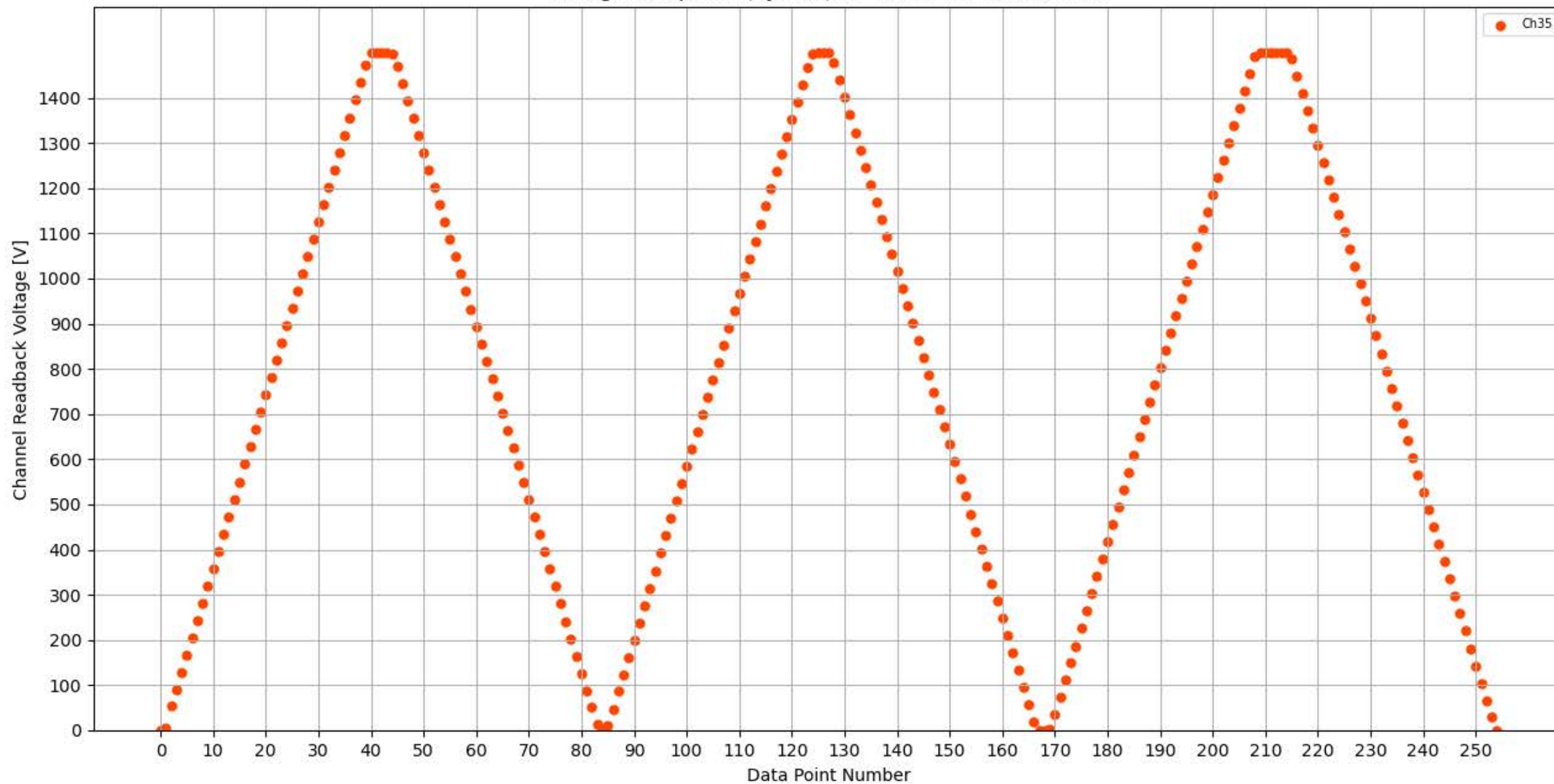
Voltage Ramp Test (Python) Bd #338, Slot #5, Ch #35
